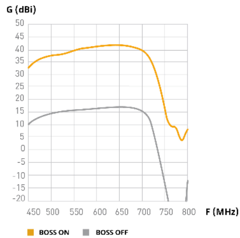
Frequency response
