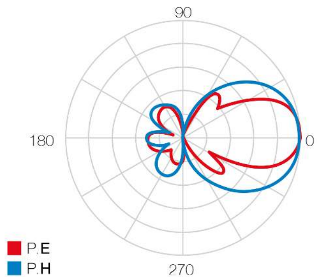
Radiation pattern
