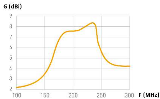
Frequenzgang
