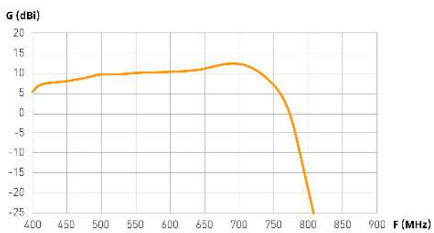
Frequency response
