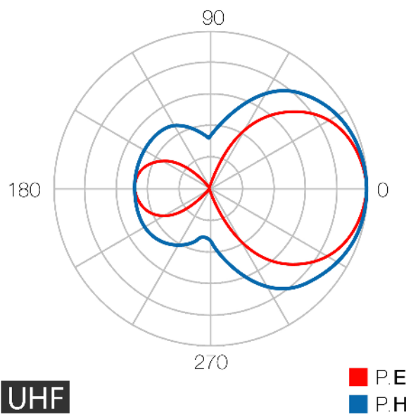
Radiation pattern
