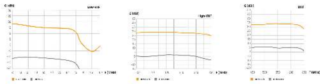
Frequency response
