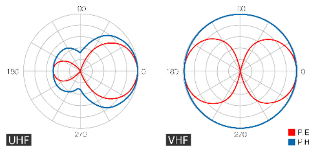
Radiation pattern
