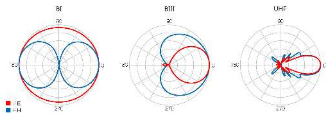
Radiation pattern
