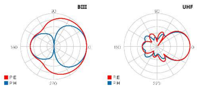
Radiation pattern
