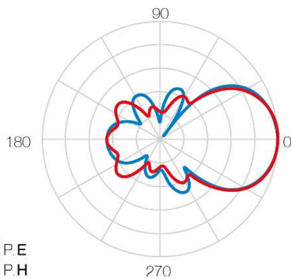
Radiation pattern
