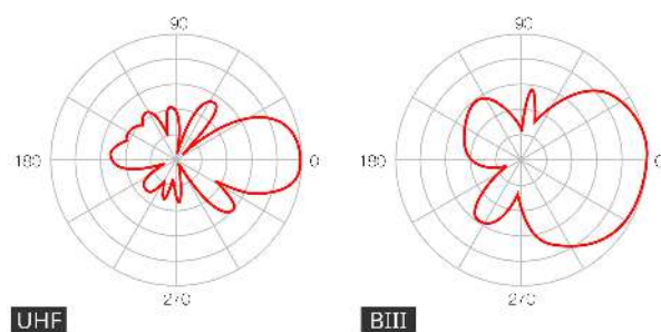
Radiation pattern
