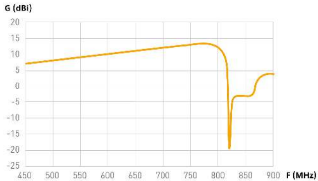
Frequenzgang
