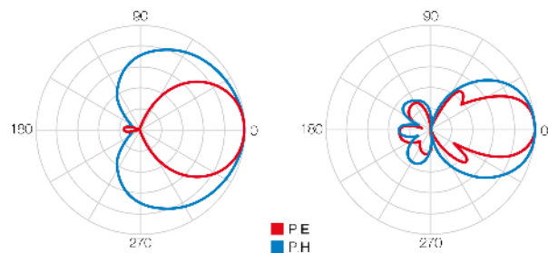
Radiation pattern
