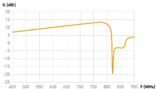
Frequency response
