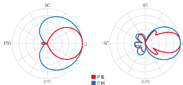
Radiation pattern
