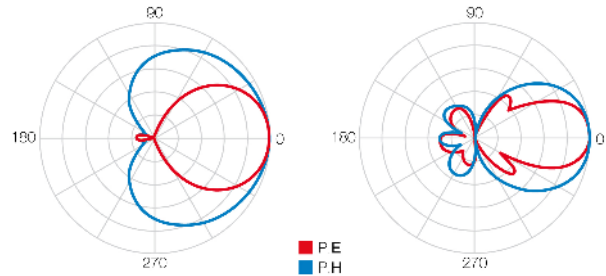
Radiation pattern
