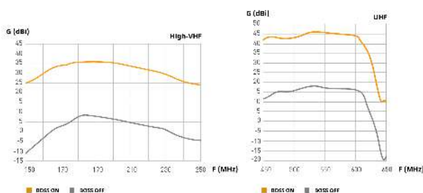
Frequency response
