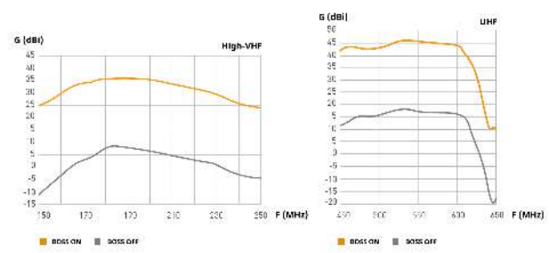
Radiation pattern
