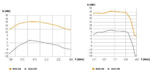
Radiation pattern
