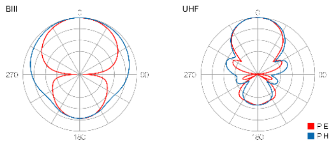
Radiation pattern
