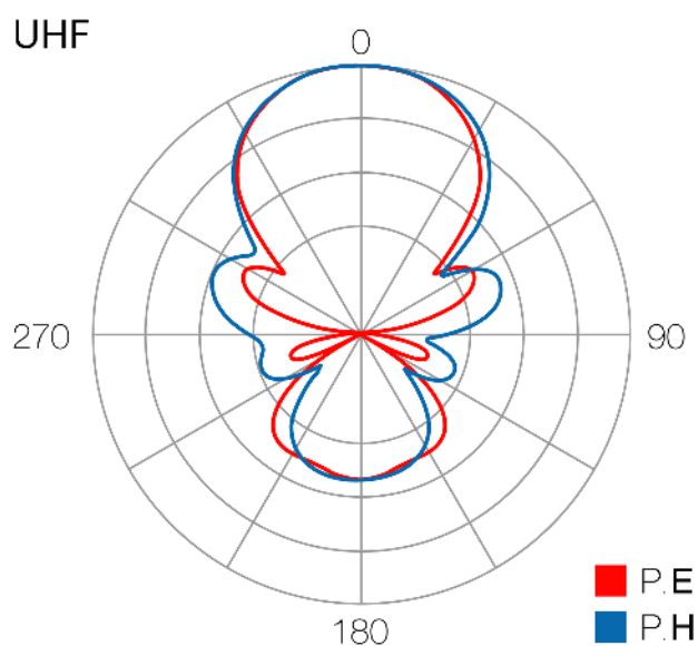
Radiation pattern
