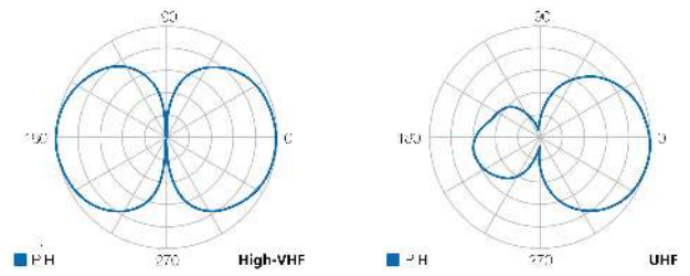
Radiation pattern
