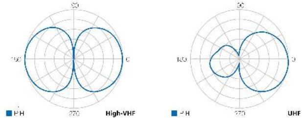
Radiation pattern
